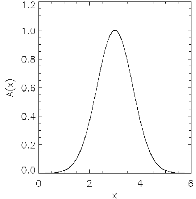
gaussoid function
