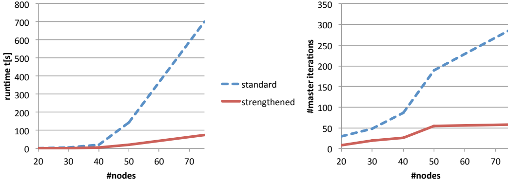
Figure 2: Comparison of the runtime (grouped by the number of nodes) and number of master iterations between two-stage branch&cut with standard and with strengthened L-shaped cuts, respectively.
