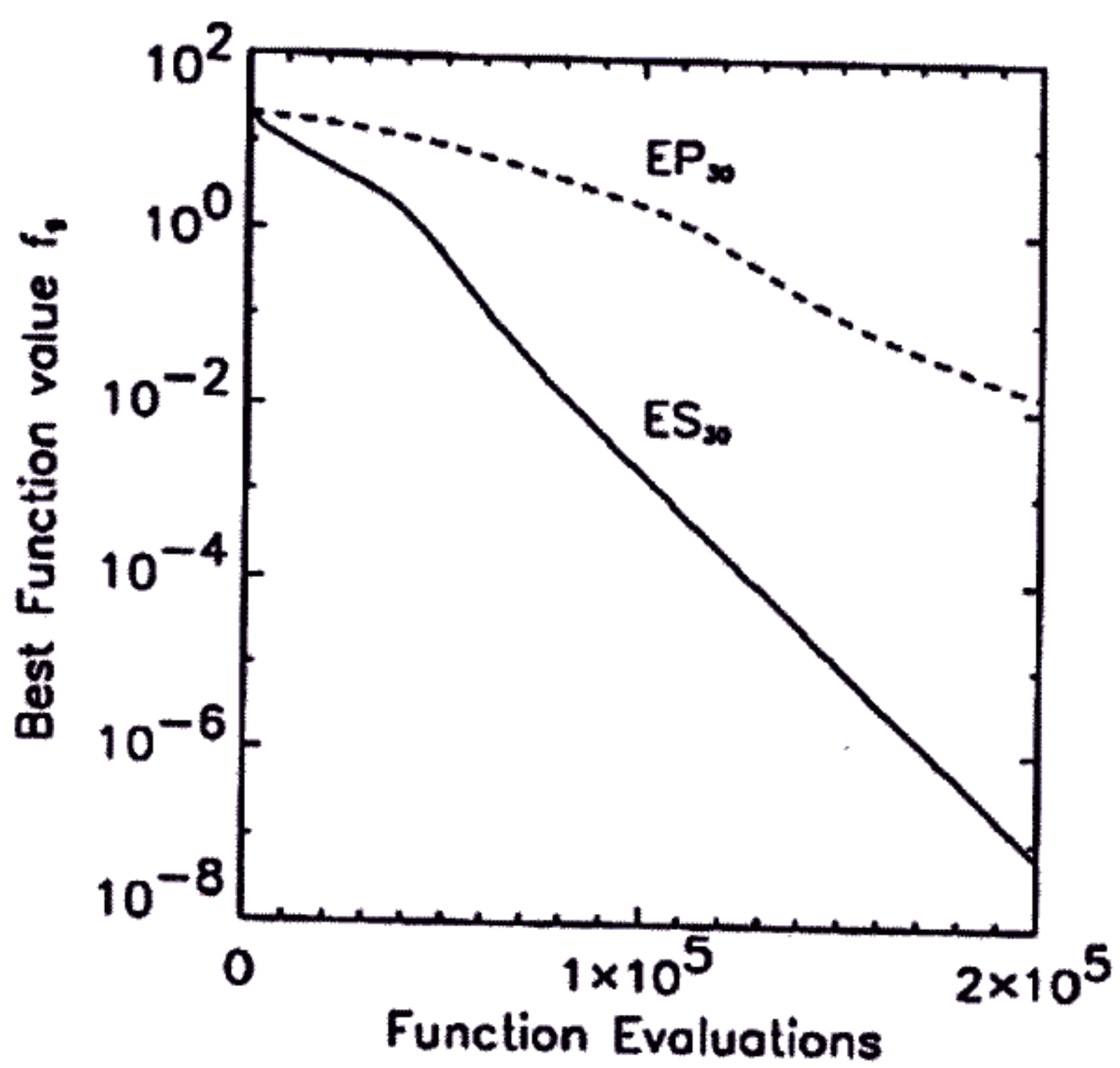
Figure 3: Experimental runs of an evolution strategy and evolutionary programming on f_b .
